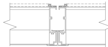
Visible Vertical Mullion
